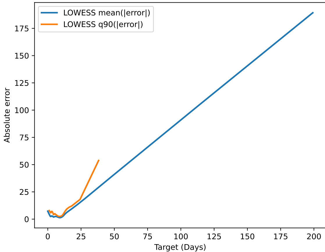
BPIC20DD: Residual trend vs Target
