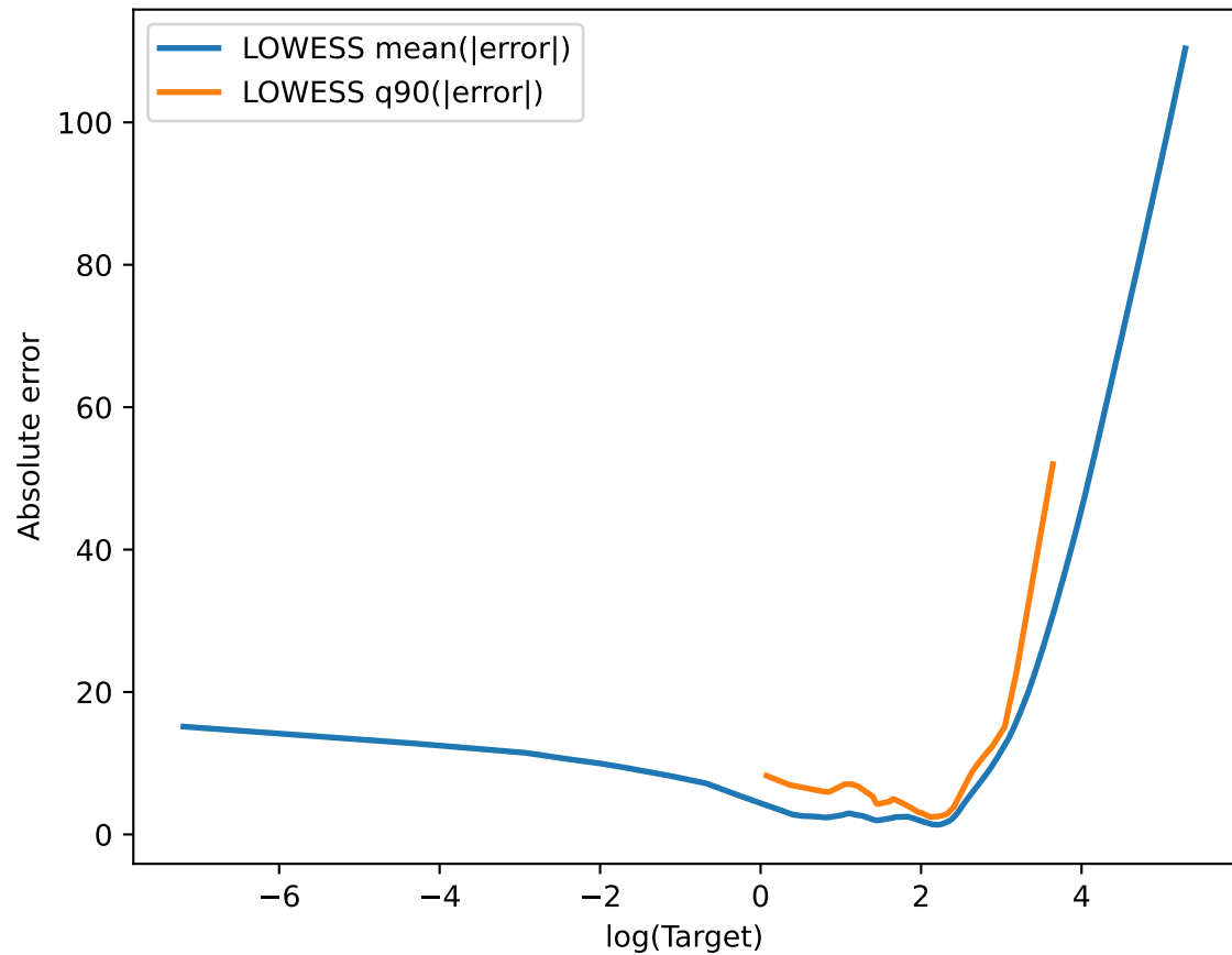
BPIC20DD: Residual trend vs log(Target)
